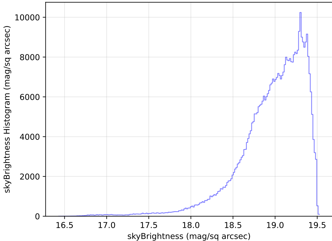
too_elab_heavy_r64_d2_gz_v3.4_10yrs All sky z band: skyBrightness Histogram
