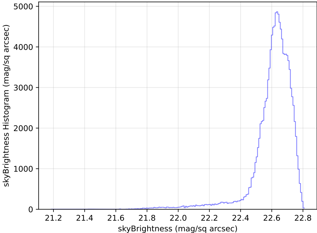
too_elab_heavy_r64_d2_gz_v3.4_10yrs All sky u band: skyBrightness Histogram
