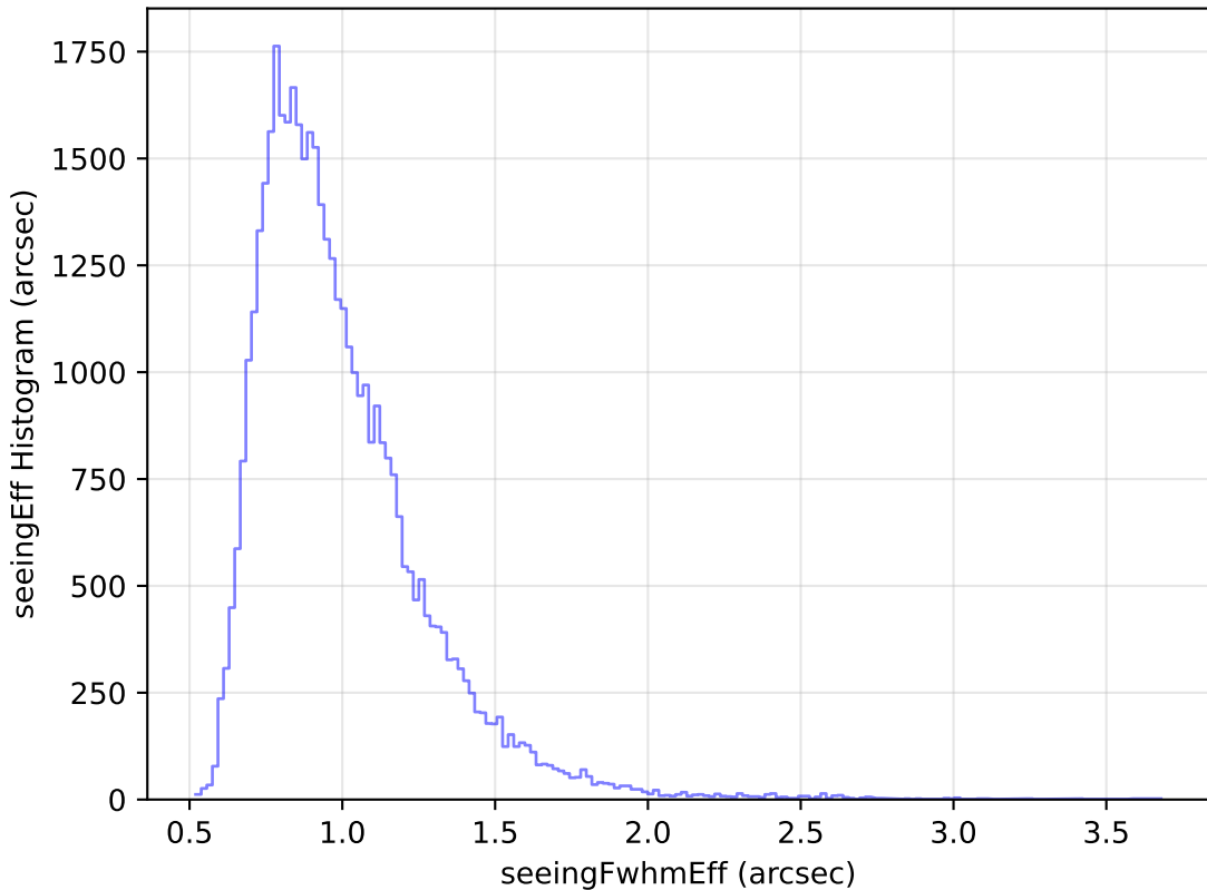
too_elab_heavy_r64_d2_gz_v3.4_10yrs Yr 1 z band: seeingEff Histogram
