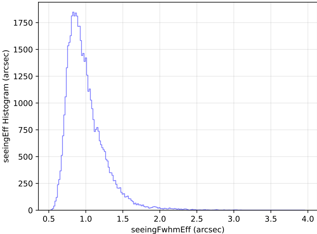
too_elab_heavy_r64_d2_gz_v3.4_10yrs Yr 1 y band: seeingEff Histogram
