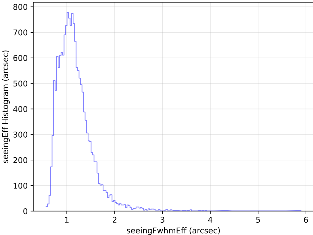
too_elab_heavy_r64_d2_gz_v3.4_10yrs Yr 1 u band: seeingEff Histogram
