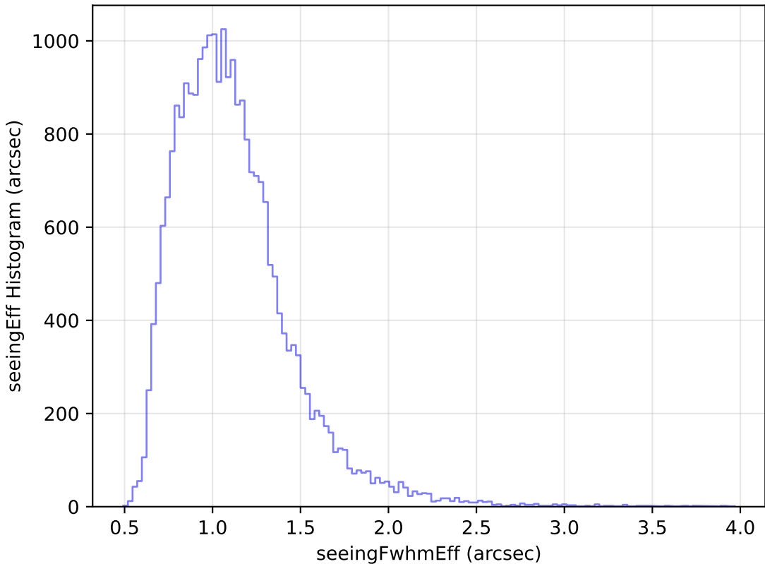
too_elab_heavy_r64_d2_gz_v3.4_10yrs Yr 1 g band: seeingEff Histogram
