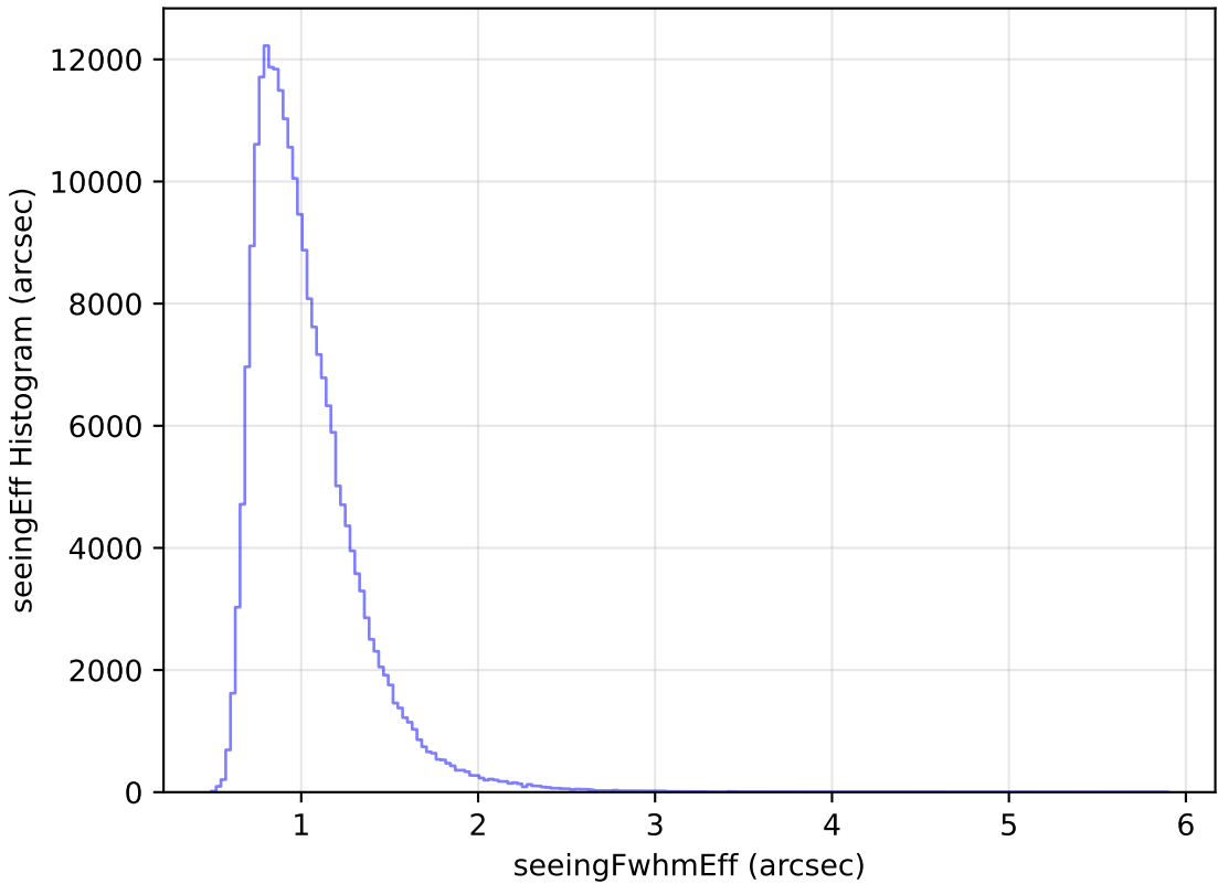
too_elab_heavy_r64_d2_gz_v3.4_10yrs Yr 1 all bands: seeingEff Histogram
