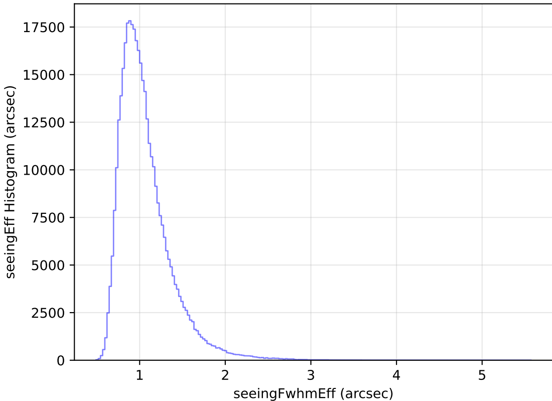
too_elab_heavy_r64_d2_gz_v3.4_10yrs WFD y band: seeingEff Histogram
