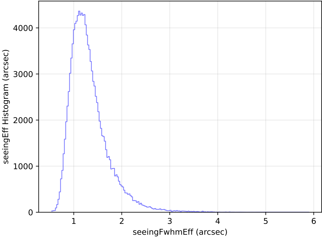
too_elab_heavy_r64_d2_gz_v3.4_10yrs WFD u band: seeingEff Histogram
