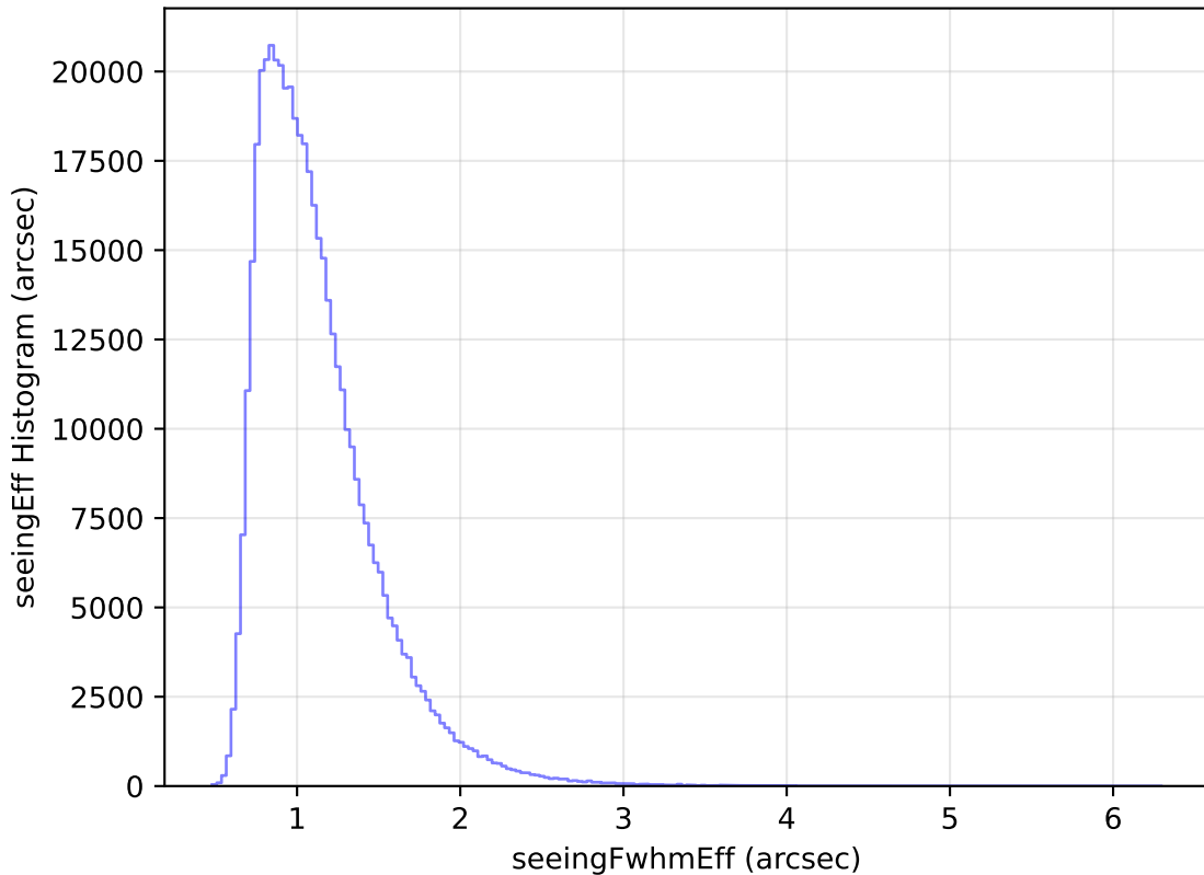
too_elab_heavy_r64_d2_gz_v3.4_10yrs WFD r band: seeingEff Histogram
