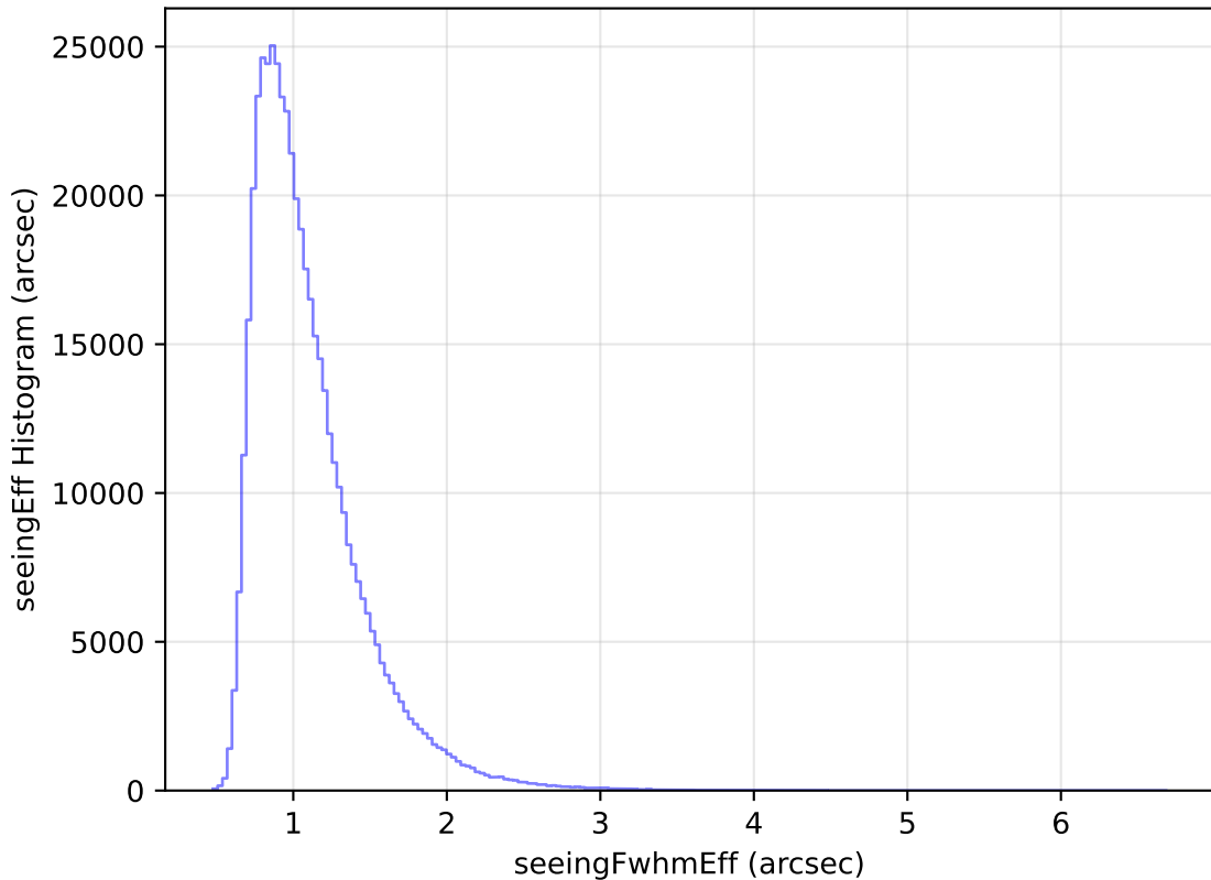
too_elab_heavy_r64_d2_gz_v3.4_10yrs WFD i band: seeingEff Histogram
