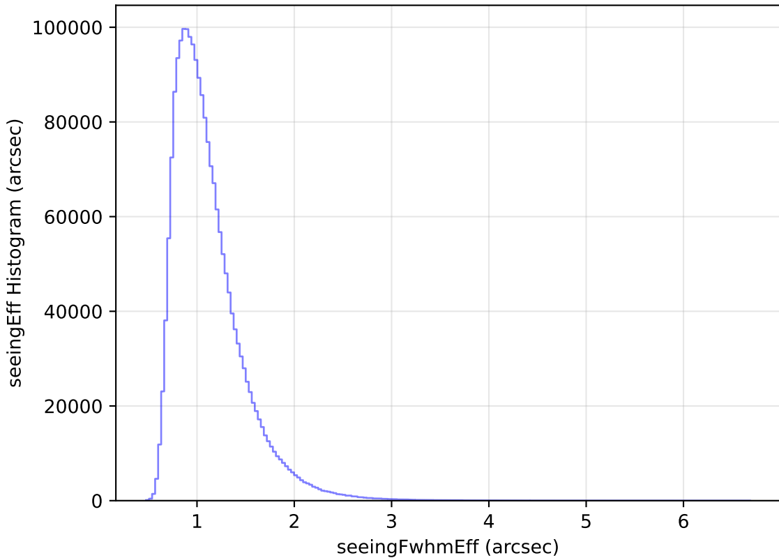
too_elab_heavy_r64_d2_gz_v3.4_10yrs WFD all bands: seeingEff Histogram
