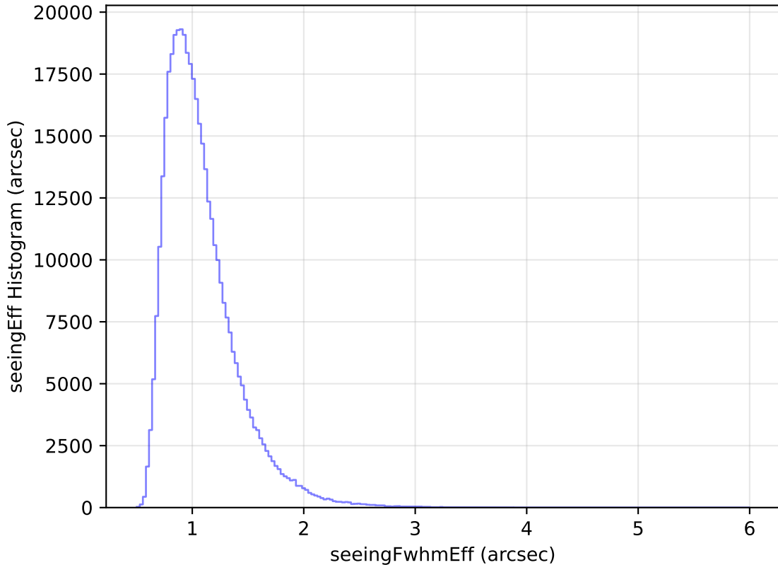
too_elab_heavy_r64_d2_gz_v3.4_10yrs All sky z band: seeingEff Histogram
