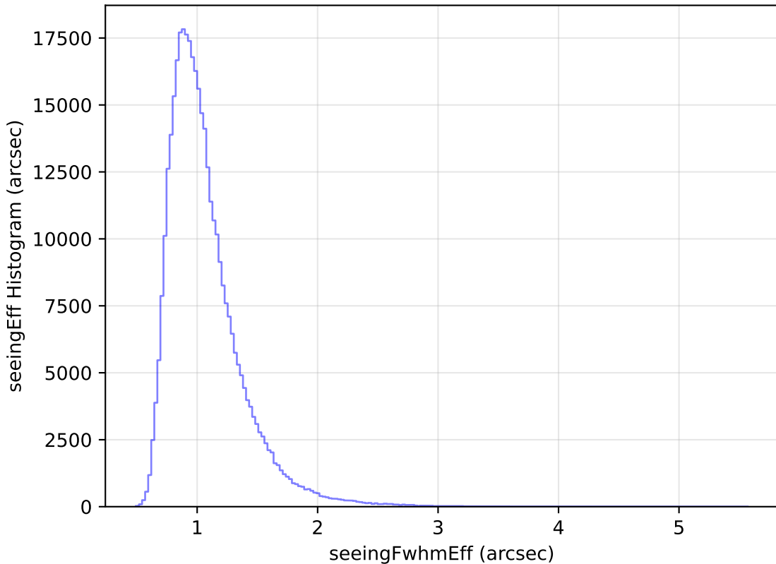
too_elab_heavy_r64_d2_gz_v3.4_10yrs All sky y band: seeingEff Histogram
