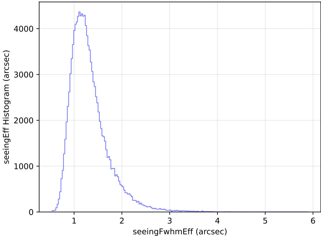
too_elab_heavy_r64_d2_gz_v3.4_10yrs All sky u band: seeingEff Histogram
