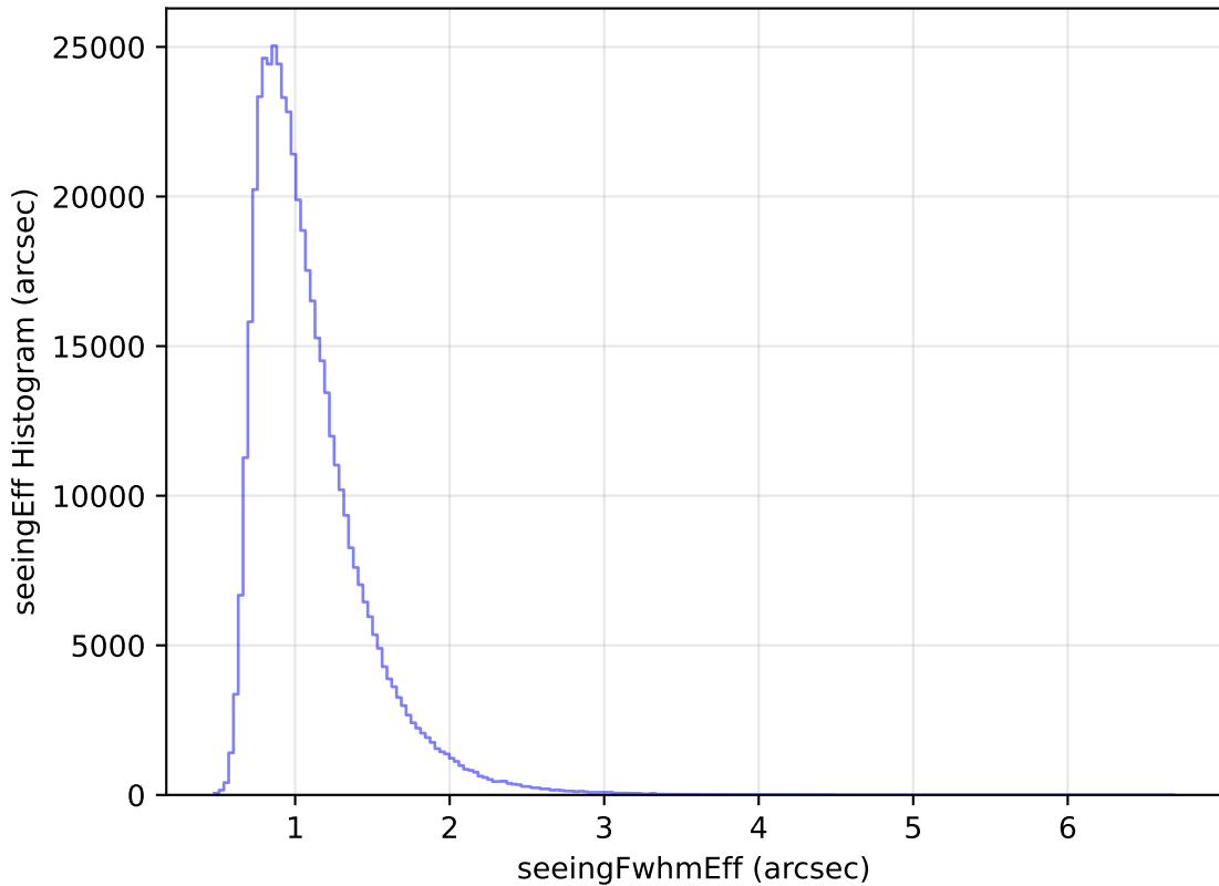
too_elab_heavy_r64_d2_gz_v3.4_10yrs All sky i band: seeingEff Histogram
