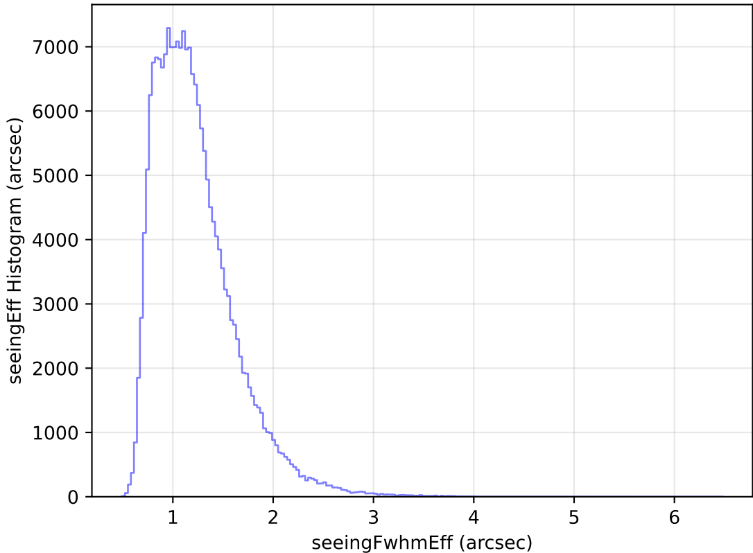
too_elab_heavy_r64_d2_gz_v3.4_10yrs All sky g band: seeingEff Histogram
