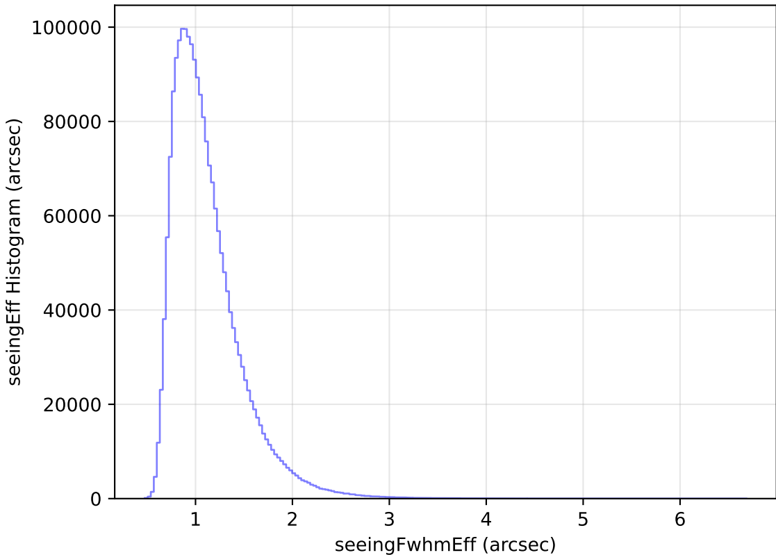
too_elab_heavy_r64_d2_gz_v3.4_10yrs All sky all bands: seeingEff Histogram
