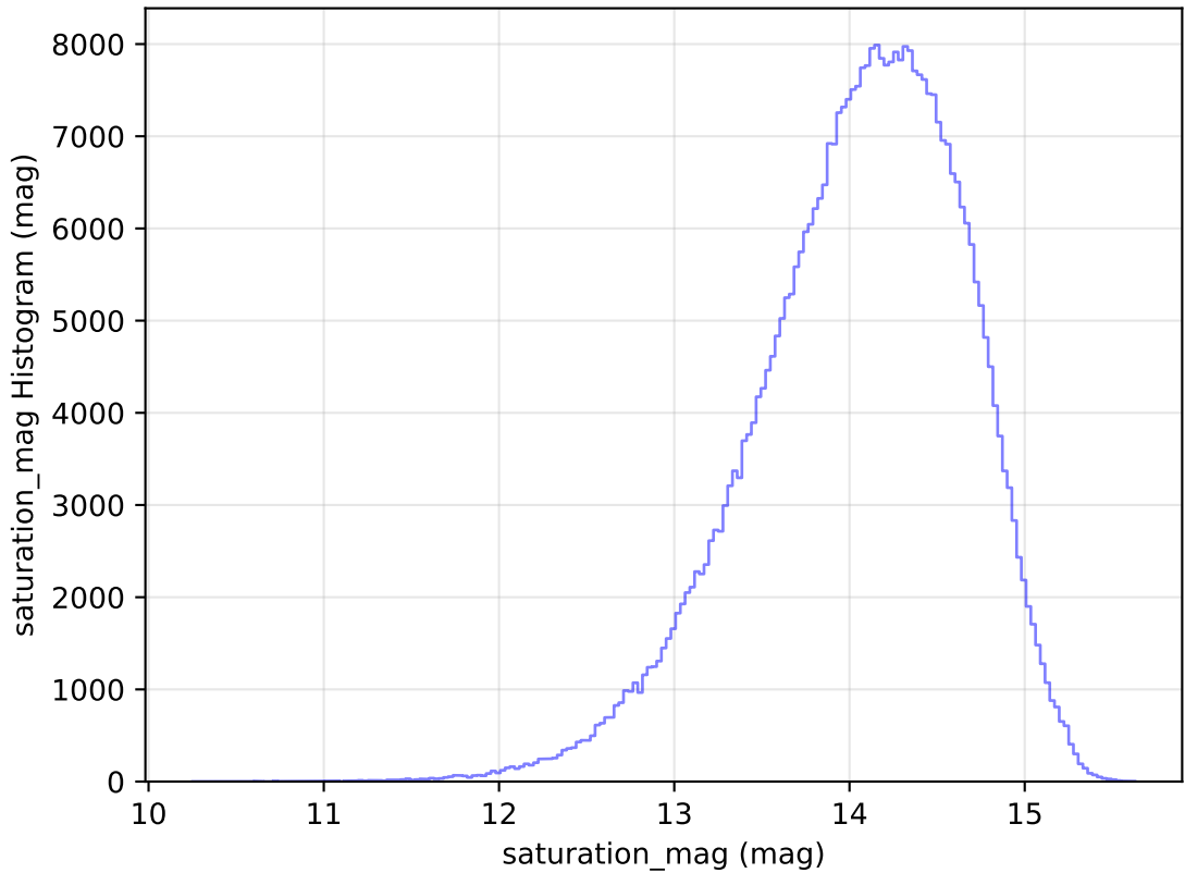
too_elab_heavy_r64_d2_gz_v3.4_10yrs WFD z band: saturation_mag Histogram
