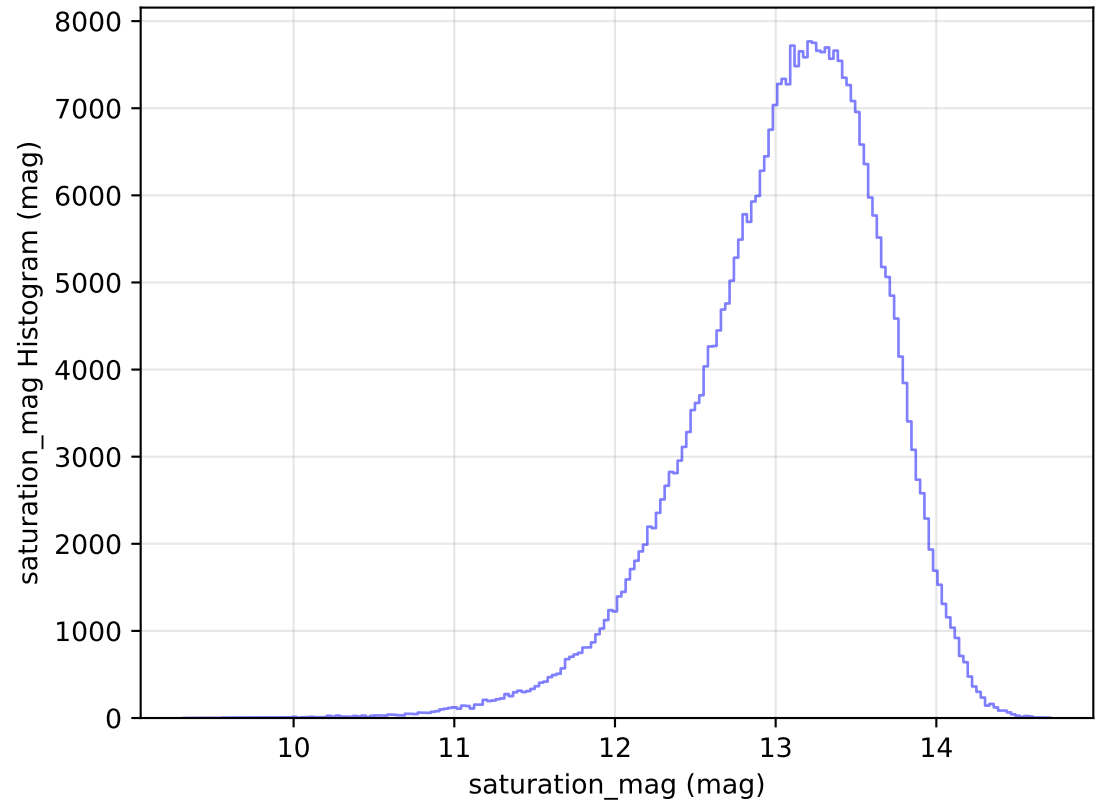
too_elab_heavy_r64_d2_gz_v3.4_10yrs WFD y band: saturation_mag Histogram
