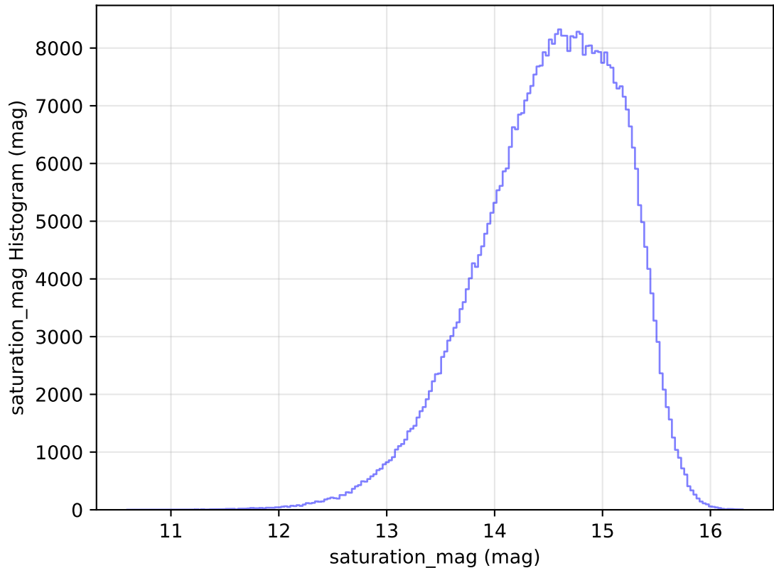
too_elab_heavy_r64_d2_gz_v3.4_10yrs WFD r band: saturation_mag Histogram
