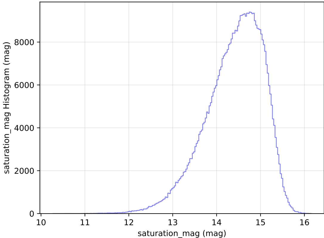
too_elab_heavy_r64_d2_gz_v3.4_10yrs WFD i band: saturation_mag Histogram
