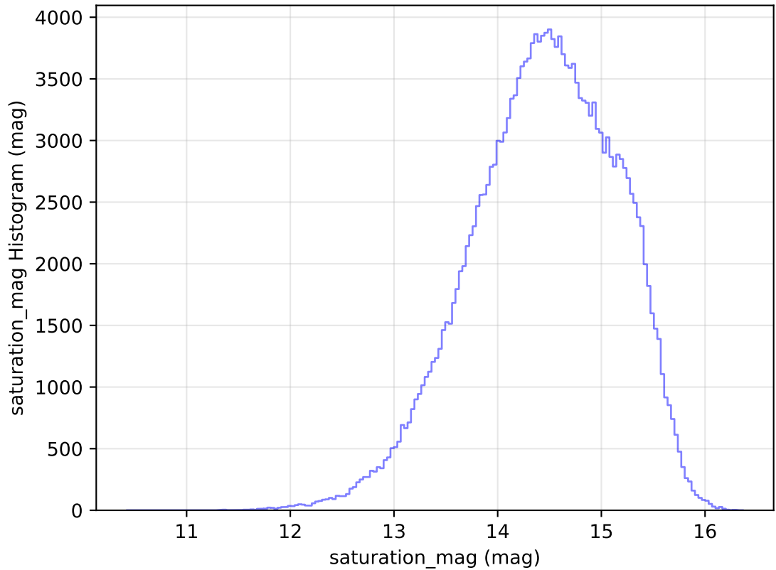
too_elab_heavy_r64_d2_gz_v3.4_10yrs WFD g band: saturation_mag Histogram
