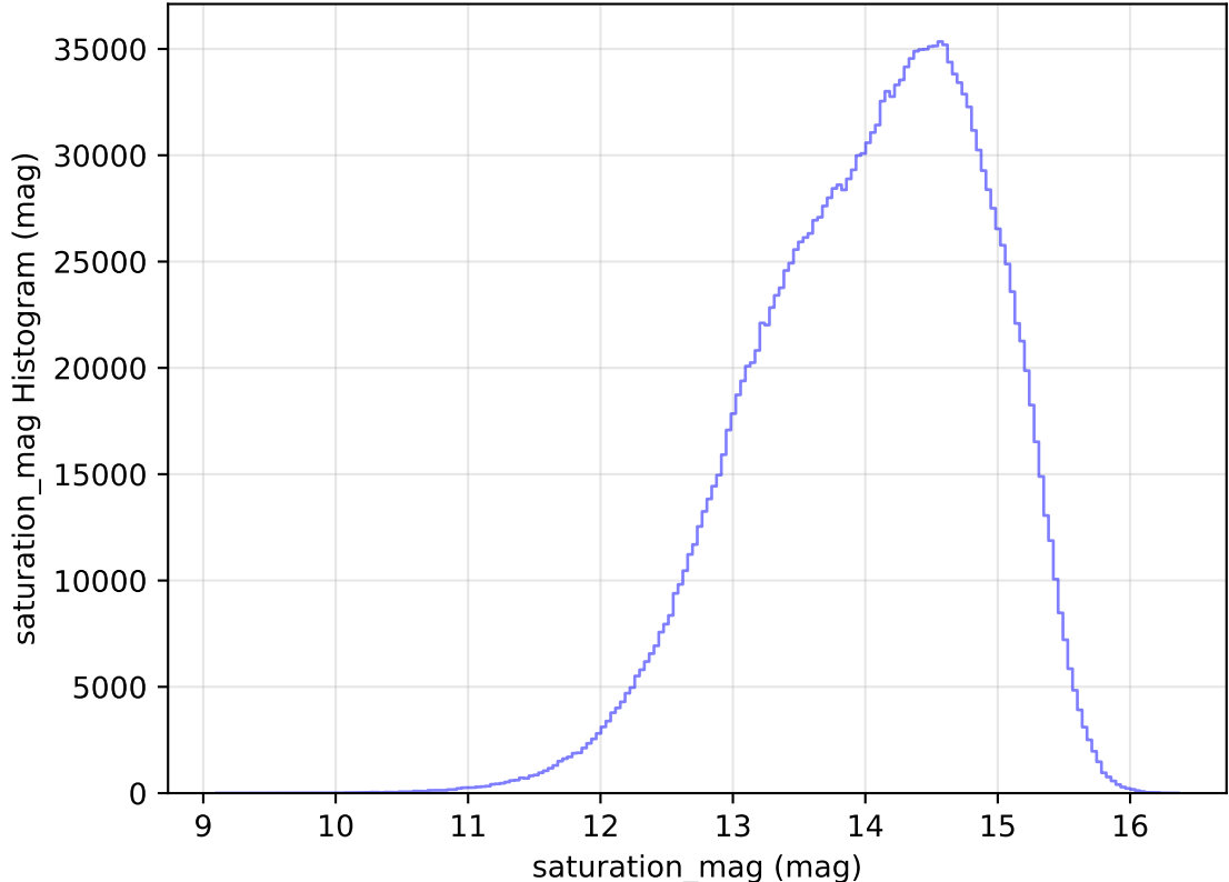
too_elab_heavy_r64_d2_gz_v3.4_10yrs WFD all bands: saturation_mag Histogram
