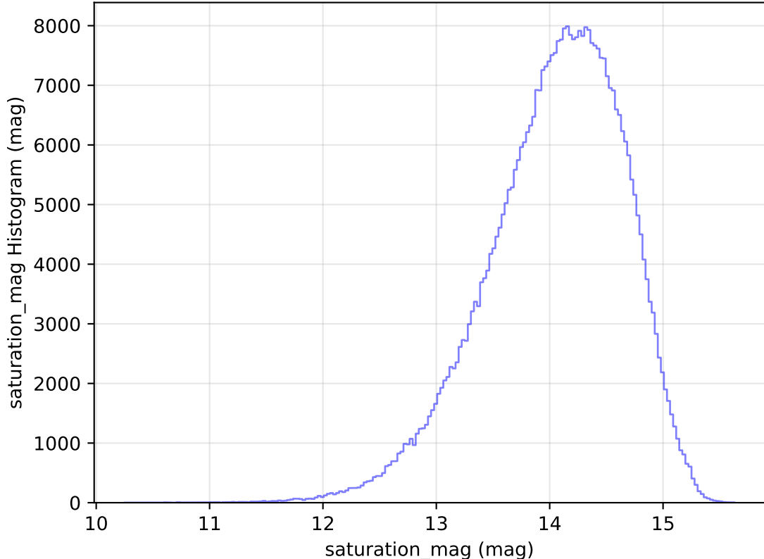
too_elab_heavy_r64_d2_gz_v3.4_10yrs All sky z band: saturation_mag Histogram
