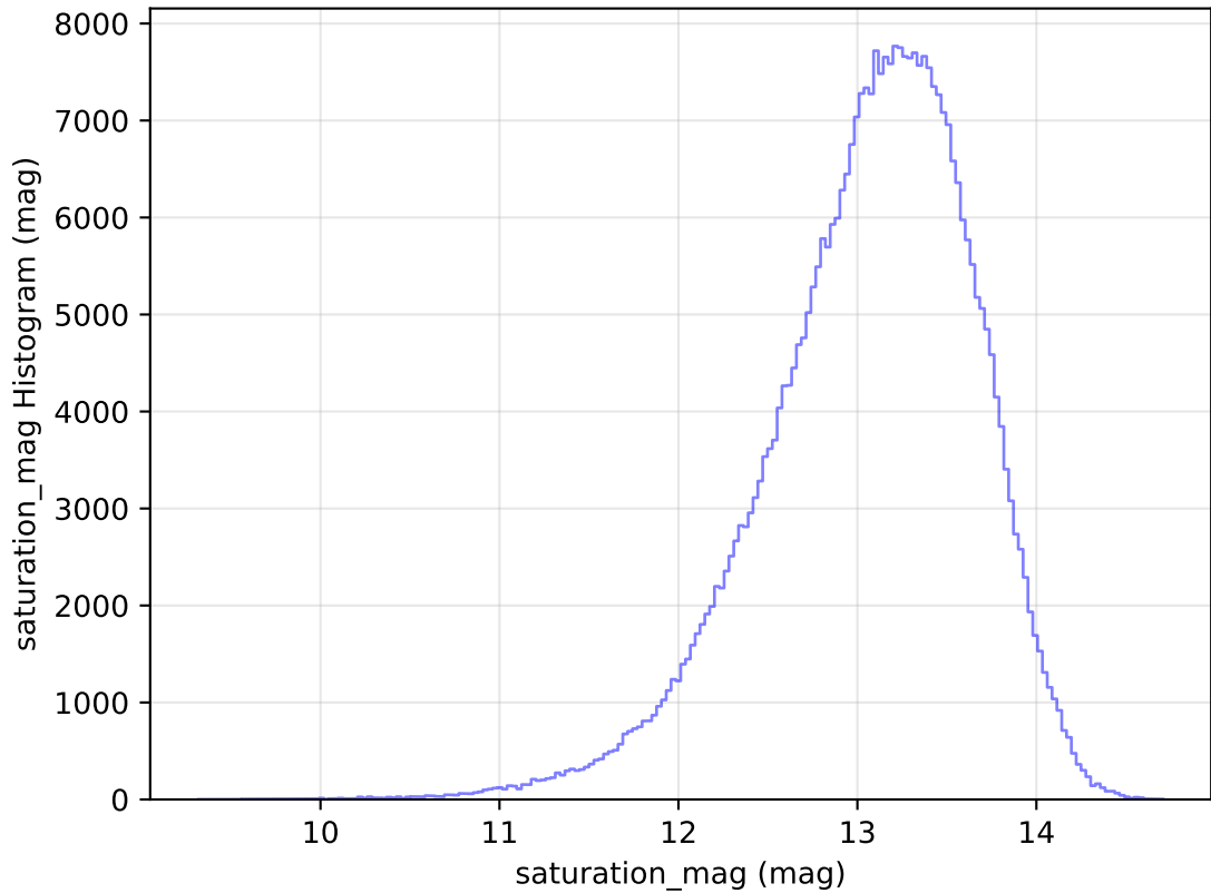
too_elab_heavy_r64_d2_gz_v3.4_10yrs All sky y band: saturation_mag Histogram
