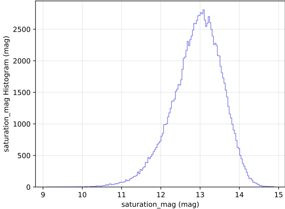
too_elab_heavy_r64_d2_gz_v3.4_10yrs All sky u band: saturation_mag Histogram
