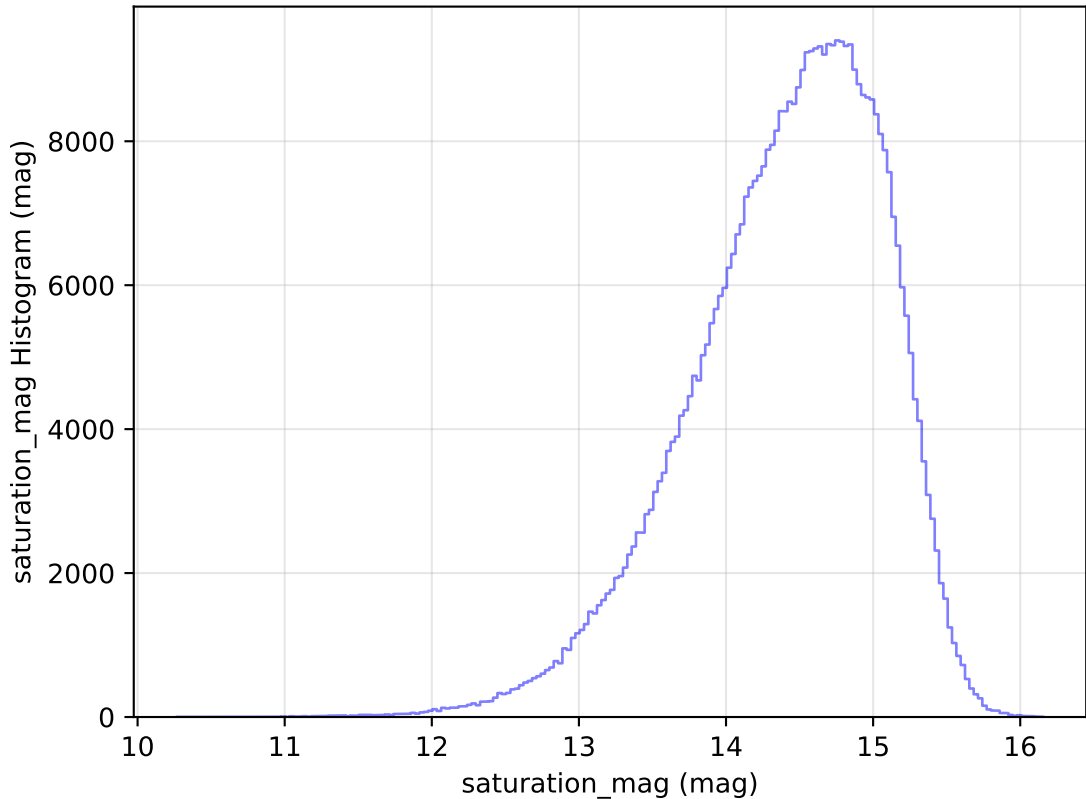
too_elab_heavy_r64_d2_gz_v3.4_10yrs All sky i band: saturation_mag Histogram
