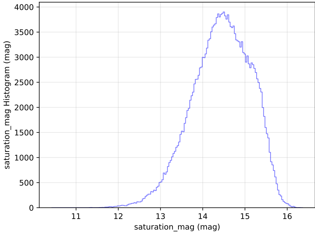
too_elab_heavy_r64_d2_gz_v3.4_10yrs All sky g band: saturation_mag Histogram
