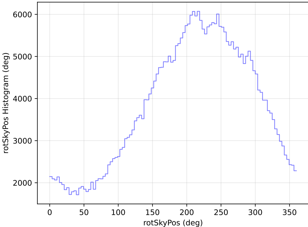
too_elab_heavy_r64_d2_gz_v3.4_10yrs WFD y band: rotSkyPos Histogram
