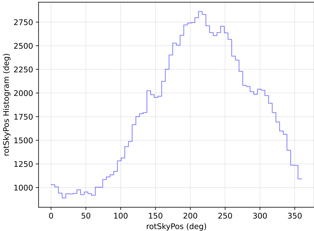
too_elab_heavy_r64_d2_gz_v3.4_10yrs WFD u band: rotSkyPos Histogram
