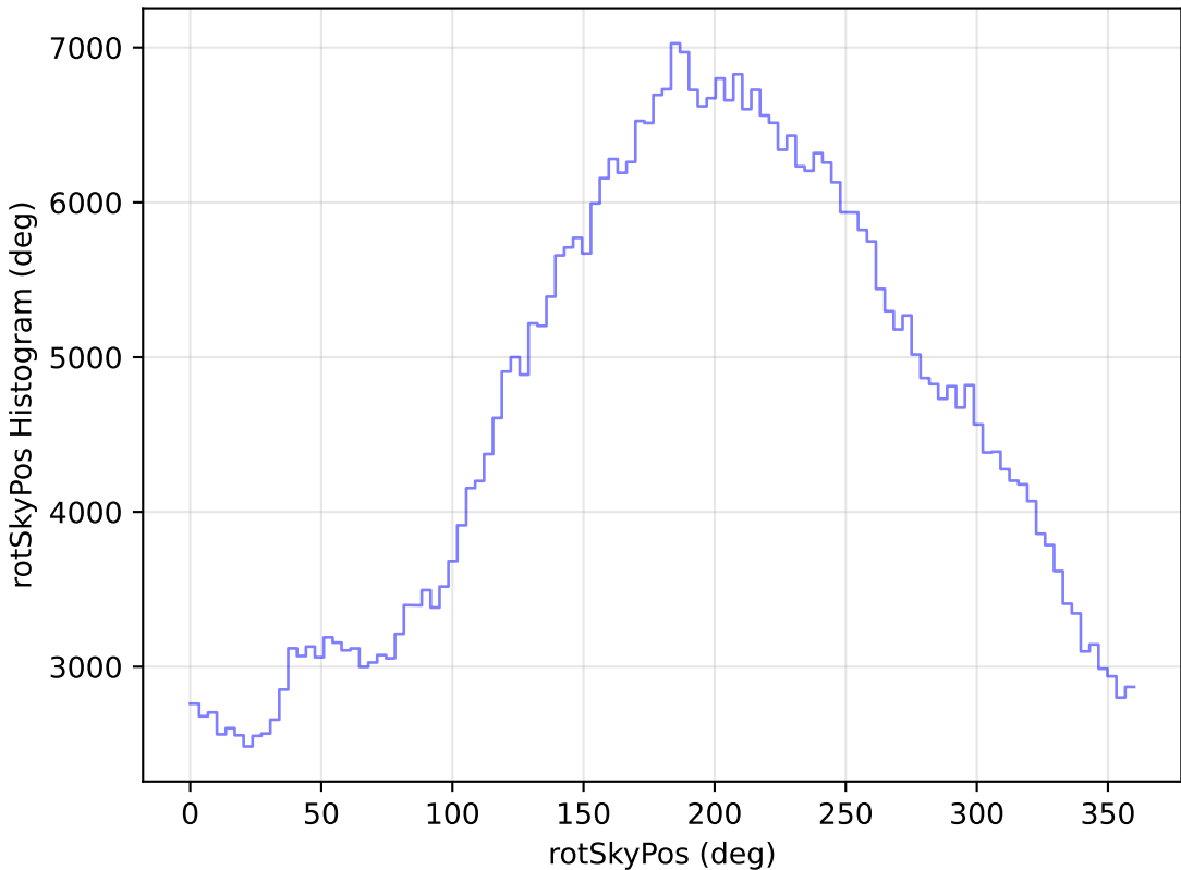
too_elab_heavy_r64_d2_gz_v3.4_10yrs WFD r band: rotSkyPos Histogram
