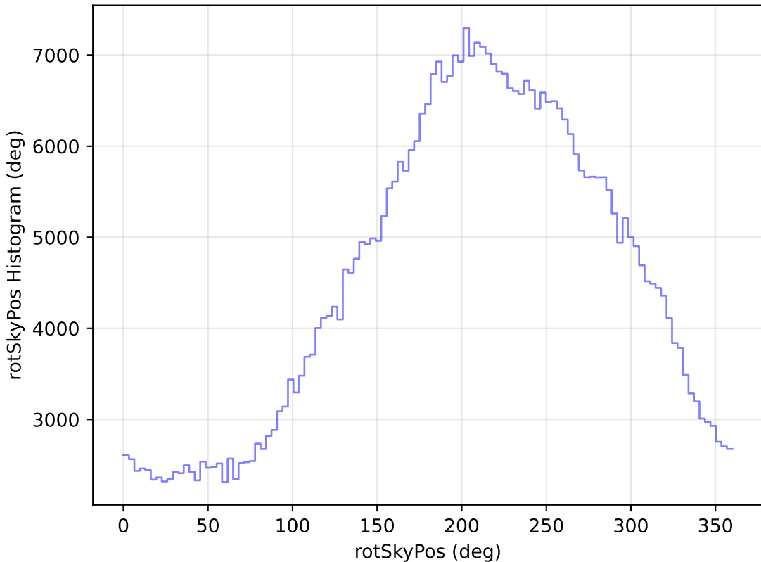
too_elab_heavy_r64_d2_gz_v3.4_10yrs WFD i band: rotSkyPos Histogram
