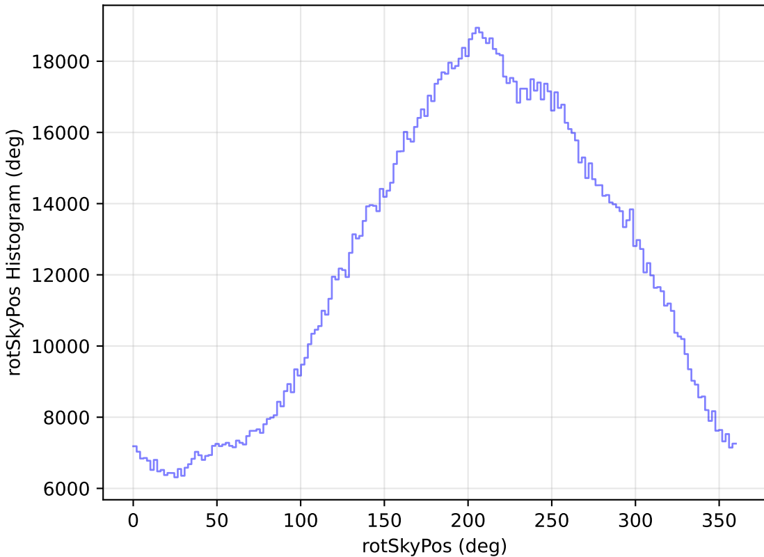
too_elab_heavy_r64_d2_gz_v3.4_10yrs WFD all bands: rotSkyPos Histogram
