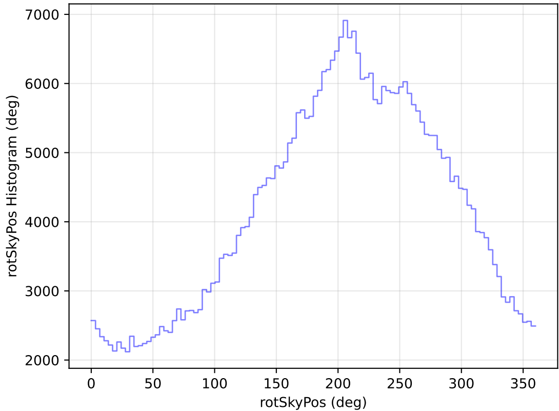
too_elab_heavy_r64_d2_gz_v3.4_10yrs All sky z band: rotSkyPos Histogram
