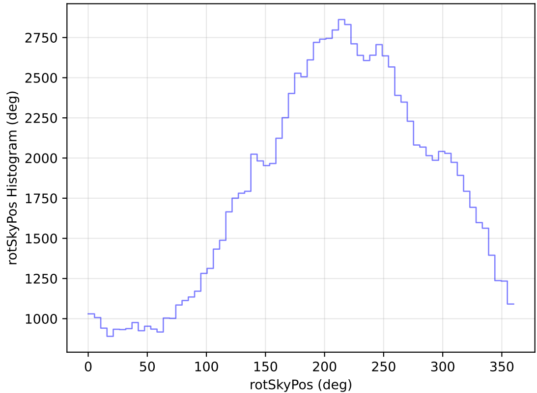
too_elab_heavy_r64_d2_gz_v3.4_10yrs All sky u band: rotSkyPos Histogram
