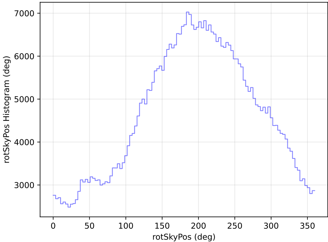
too_elab_heavy_r64_d2_gz_v3.4_10yrs All sky r band: rotSkyPos Histogram
