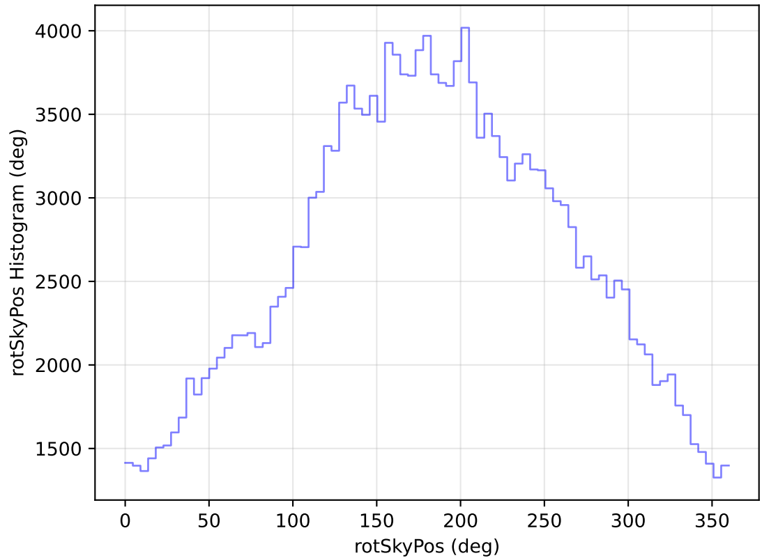
too_elab_heavy_r64_d2_gz_v3.4_10yrs All sky g band: rotSkyPos Histogram
