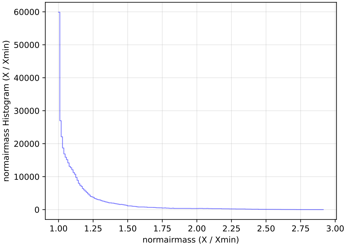
too_elab_heavy_r64_d2_gz_v3.4_10yrs WFD z band: normairmass Histogram
