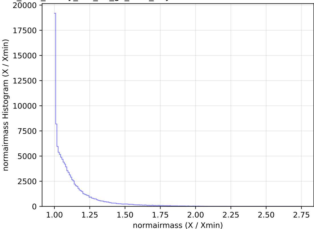
too_elab_heavy_r64_d2_gz_v3.4_10yrs WFD u band: normairmass Histogram
