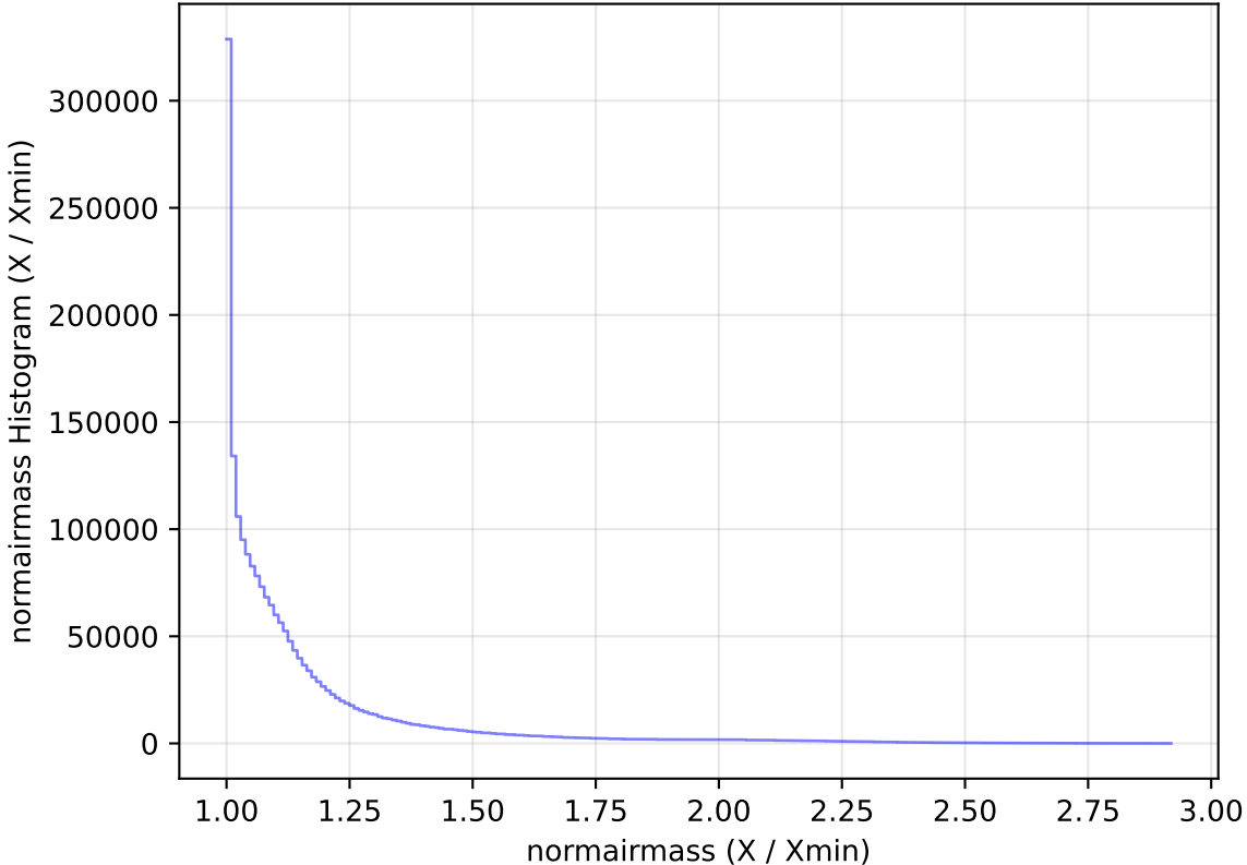
too_elab_heavy_r64_d2_gz_v3.4_10yrs WFD all bands: normairmass Histogram
