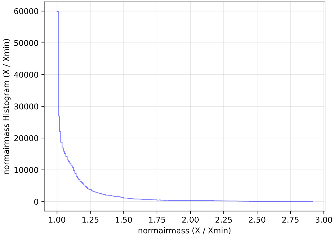
too_elab_heavy_r64_d2_gz_v3.4_10yrs All sky z band: normairmass Histogram
