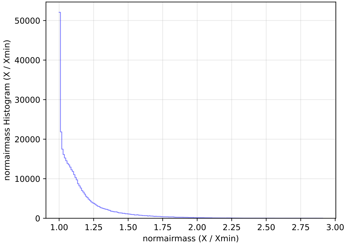
too_elab_heavy_r64_d2_gz_v3.4_10yrs All sky y band: normairmass Histogram
