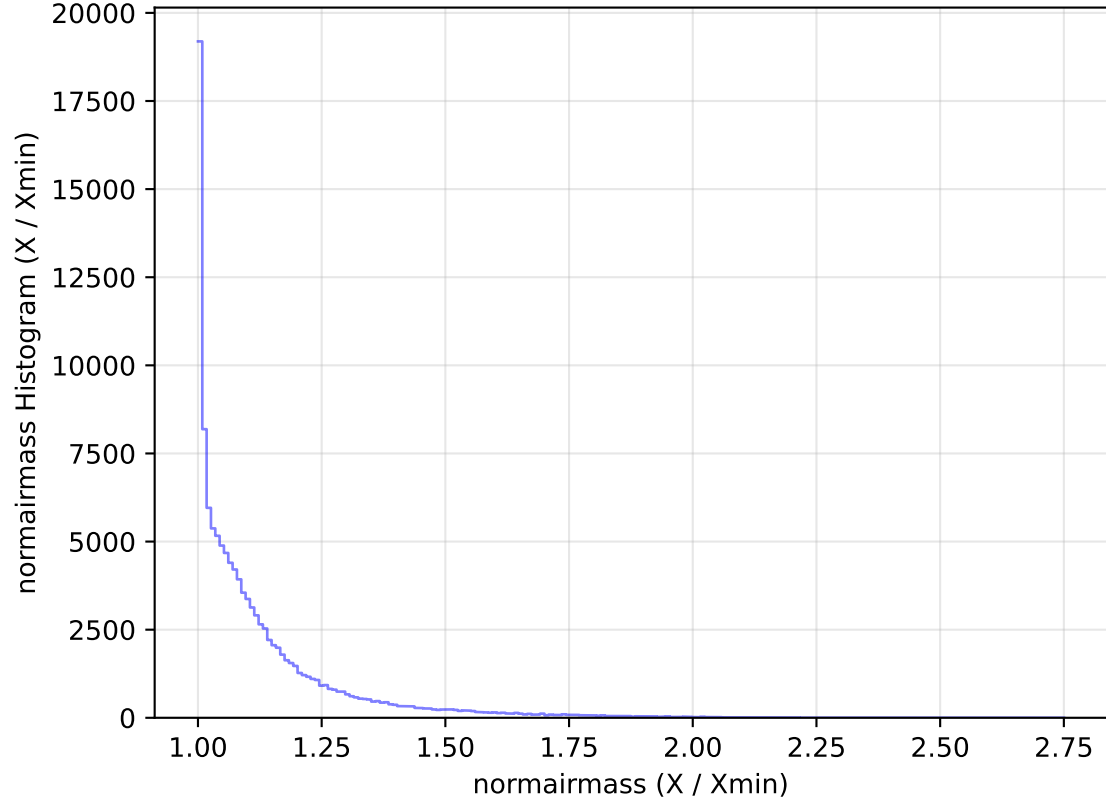
too_elab_heavy_r64_d2_gz_v3.4_10yrs All sky u band: normairmass Histogram
