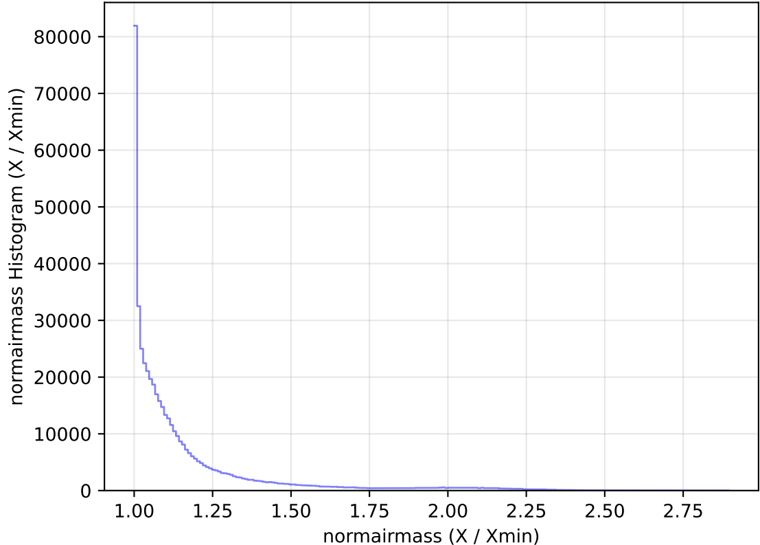
too_elab_heavy_r64_d2_gz_v3.4_10yrs All sky r band: normairmass Histogram
