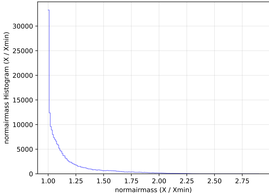
too_elab_heavy_r64_d2_gz_v3.4_10yrs All sky g band: normairmass Histogram
