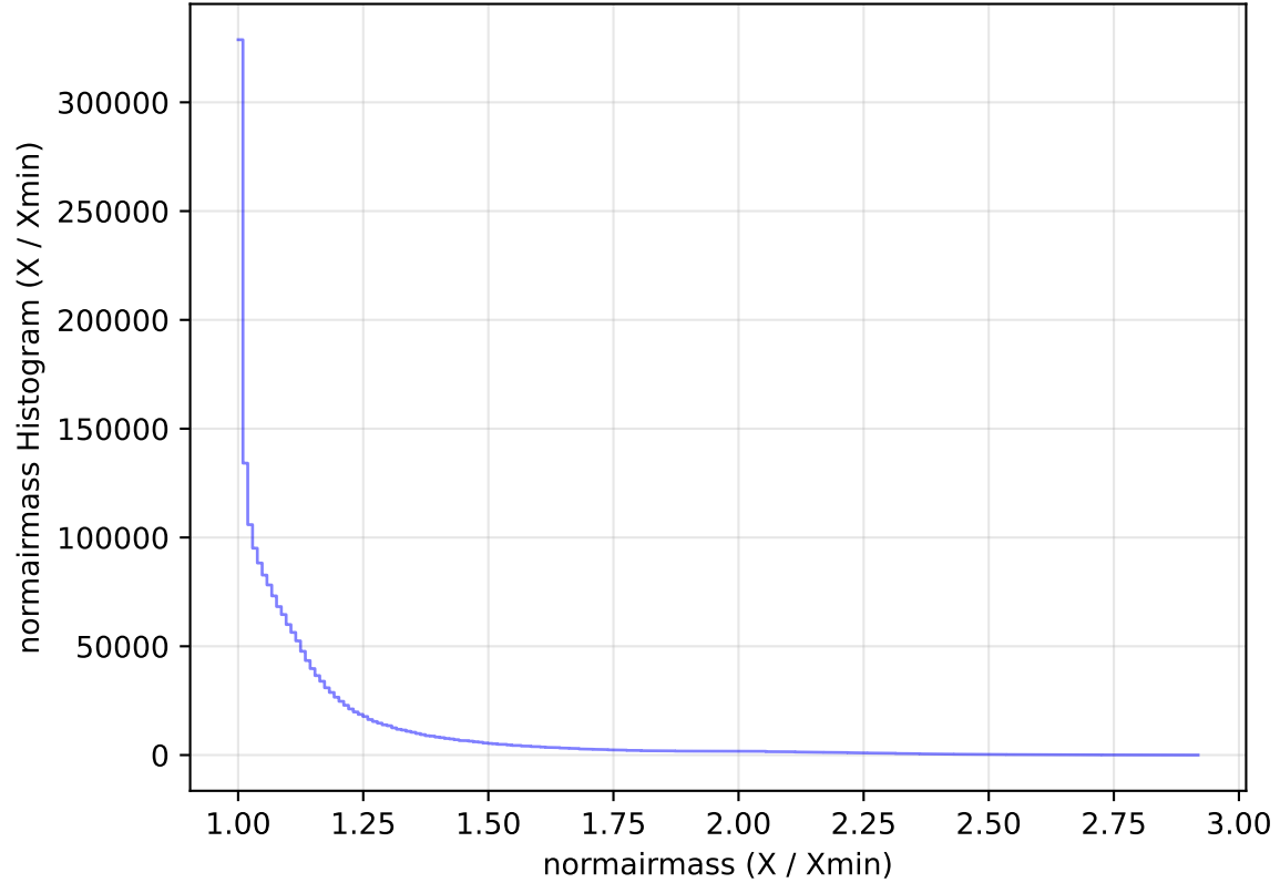
too_elab_heavy_r64_d2_gz_v3.4_10yrs All sky all bands: normairmass Histogram
