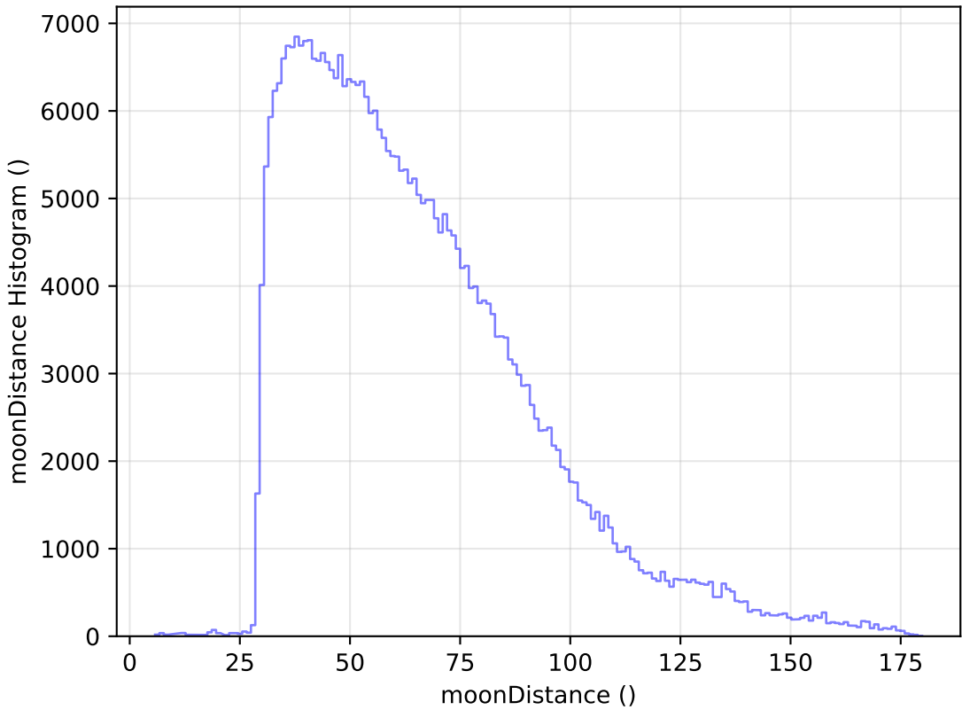
too_elab_heavy_r64_d2_gz_v3.4_10yrs WFD y band: moonDistance Histogram
