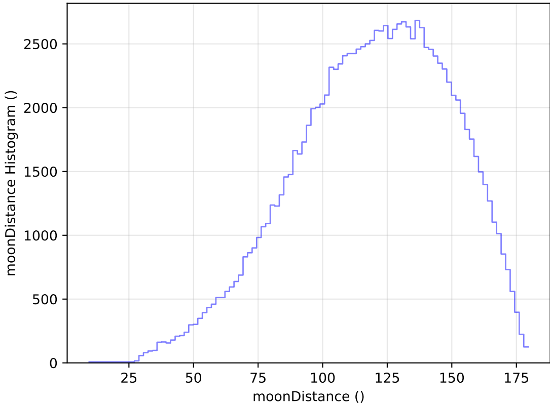
too_elab_heavy_r64_d2_gz_v3.4_10yrs WFD u band: moonDistance Histogram
