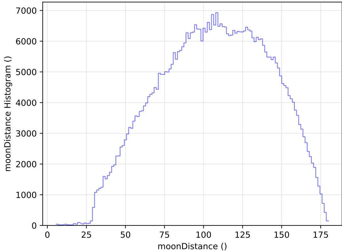
too_elab_heavy_r64_d2_gz_v3.4_10yrs WFD r band: moonDistance Histogram
